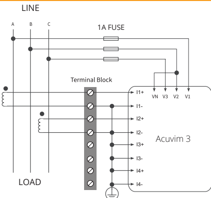
2 Element 3 Wire Delta (2LL, 2CT)
